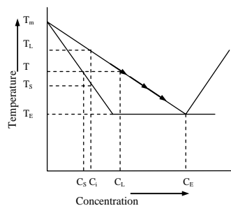
Fig. 3: A Schematic phase diagram showing the solute enrichment in the remaining liquid during solidification
