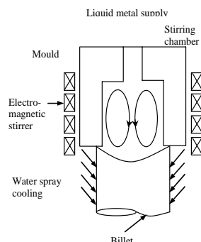
Fig. 1: Schematic diagram of an electromagnetic stirring system
